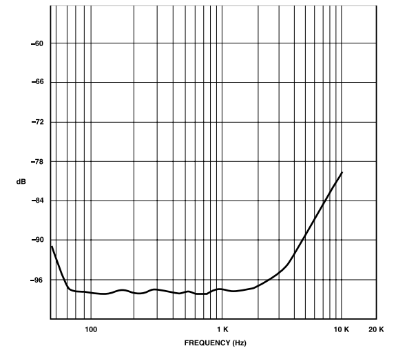
Figure 7.5 Typical Crosstalk
